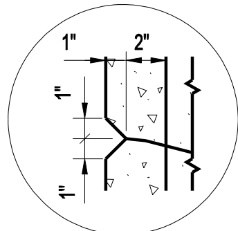
Rustication Detail
